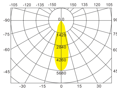
Intensity(unit:cd) Citizen 28W \theta_{av}(\frac{1}{2}):31^\circ
