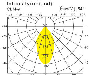
With 1021 reflector(Flood)
