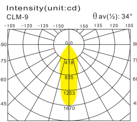
With 1028 reflector(Narrow)
