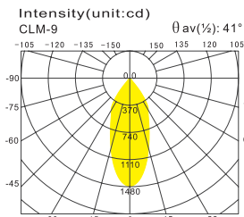
With 1128 reflector(Medium)
