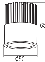
7W heatsink with H:22mm reflectors
