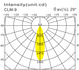
With 1017-F reflector(Narrow)
