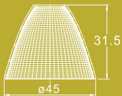
1017, 1017F
