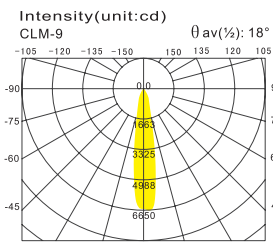
With 1017 reflector(Narrow)
